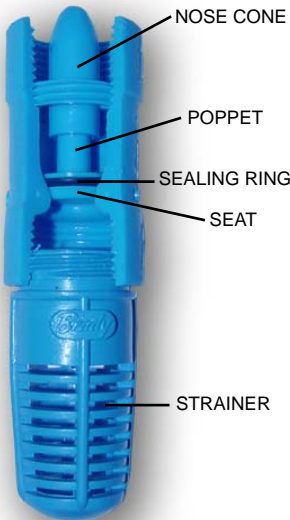
Brady Foot Valve
