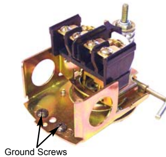
Ground Screws
